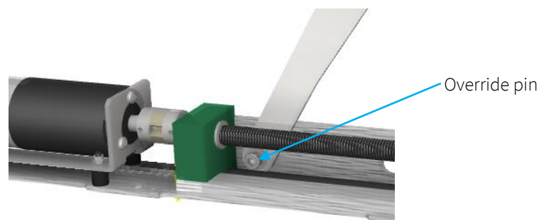
Figure 6 – Manual override bolt location
