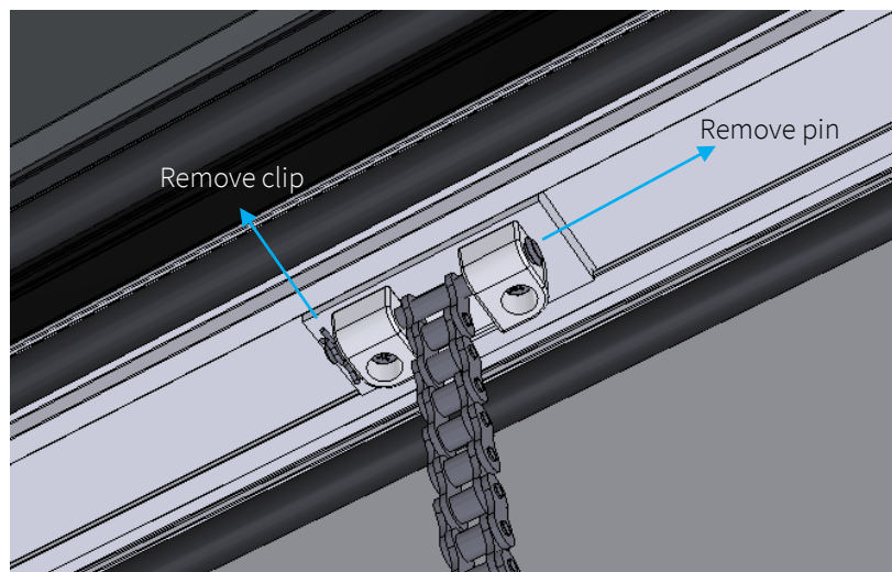
Figure 10 – Manual disconnect
