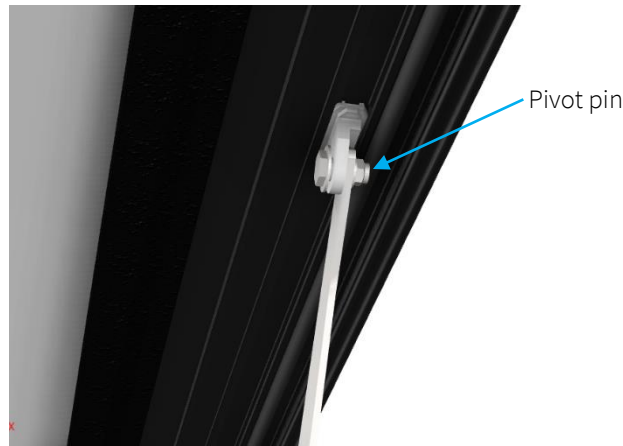
Figure 7 – Manual disconnect
